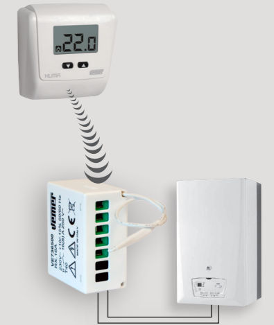
Example of connection with 1 channel remote actuator. Note: the remote actuator must be powered by mains.
