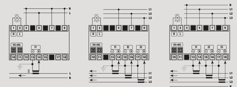
AC Single-phase
